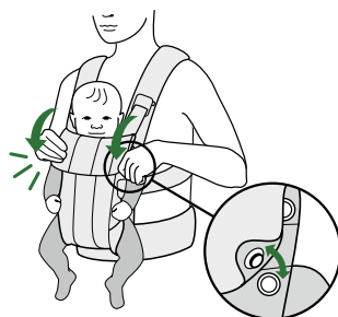
Alumine
